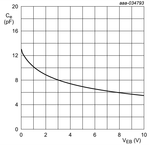
Fig. 6. Emitter capacitance as a function of emitter-base voltage; typical values
